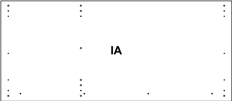
1388x605x18mm
